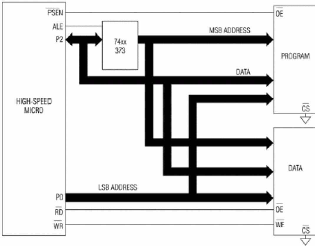
Figure 3. Page mode 2 memory interface
